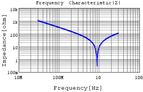
RDE5C1H5R0C0K1H03B |Z| DC0V, 25degC
