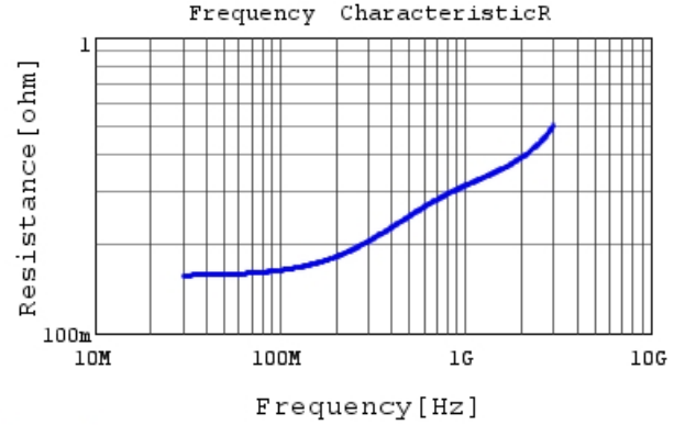
RDE5C1H5R0C0K1H03B R DC0V, 25degC
