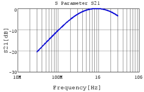
RDE5C1H5R0C0K1H03B S21 DC0V, 25degC
