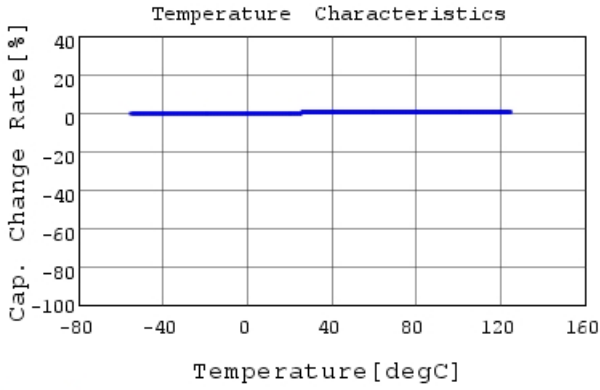
RDE5C1H5R0C0K1H03B C-Temp. capchange, DC0V,
