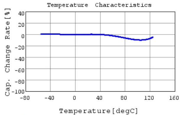
GR442QR73D331KW01 C-Temp. capchange, DCOV, 1
