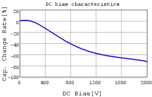
GR442QR73D331KW01 C-DC bias capchange, 25.0c
