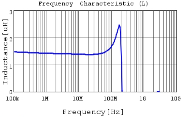
LQH32NH1R5J23 L
