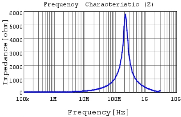
LQH32NH1R5J23 |Z|
