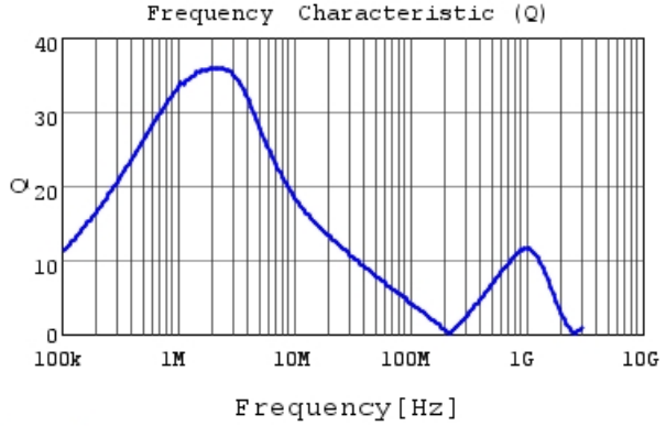
LQH32NH1R5J23 Q
