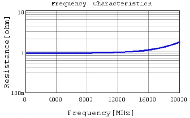
GRM0335C2AR50BA01 R DCOV, 25degC
