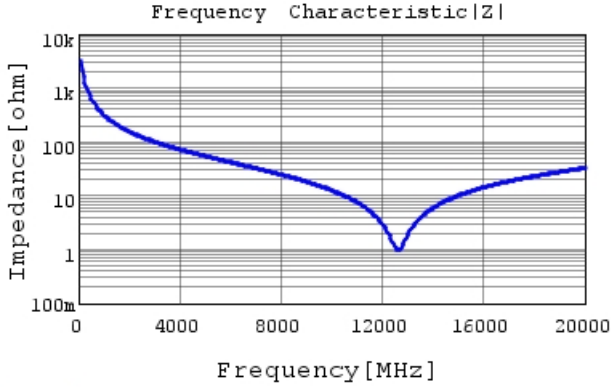
GRM0335C2AR50BA01 |Z| DCOV, 25degC
