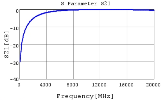
GRM0335C2AR50BA01 S21 DCOV, 25degC
