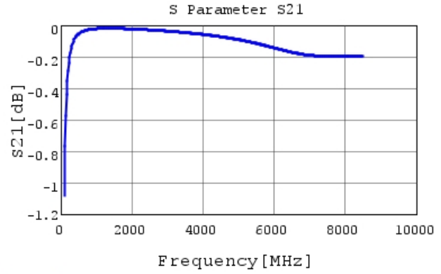
GRM0335C1H300GA01 S21 DCOV, 25degC
