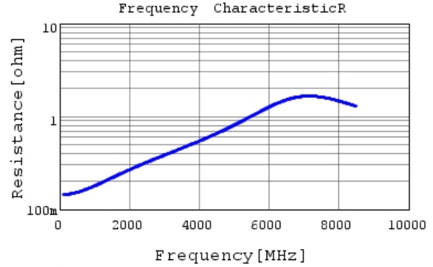
GRM0335C1H300GA01 R DCOV, 25degC
