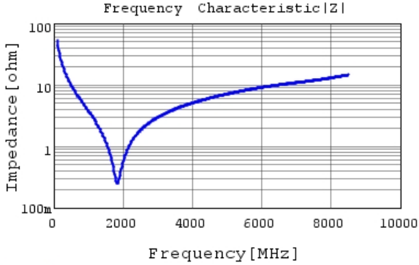
GRM0335C1H300GA01 |Z| DCOV, 25degC
