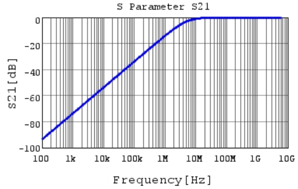
GCM033R71E331KA03 S21 DC0V, 25degC
