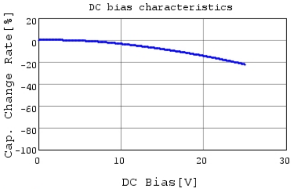
GCM033R71E331KA03 C-DC bias capchange, 25.0c
