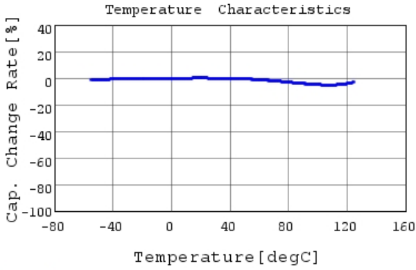
GCM033R71E331KA03 C-Temp. capchange, DC0.0V,
