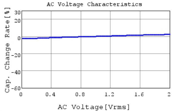
GCM033R71E331KA03 C-AC Voltage capchange, Dc
