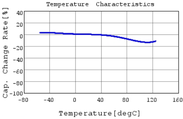
RDER72J104K4K1H03B C-Temp. capchange, DCOV,
