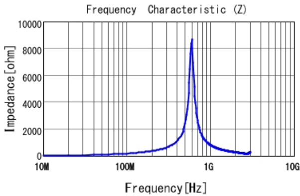
LQP03TNR27J02 |Z|
