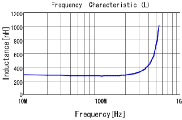
LQP03TNR27J02 L
