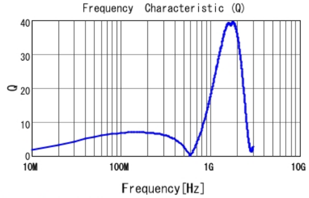
LQP03TNR27J02 Q
