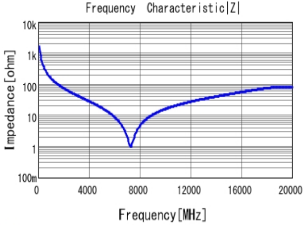
■ GRM1555C1H1R0CA01 |Z| DCOV, 25degC
