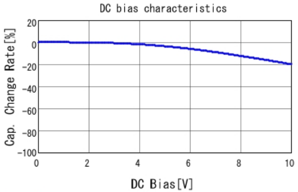
GRM319R61A225KA01 C-DC bias capchange, 25.0degC, A
