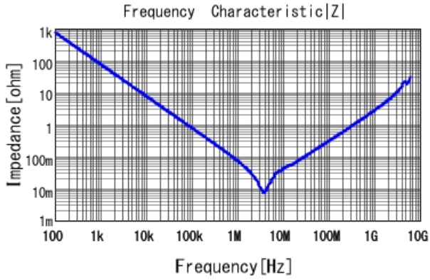
GRM319R61A225KA01 |Z| DCOV, 25degC
