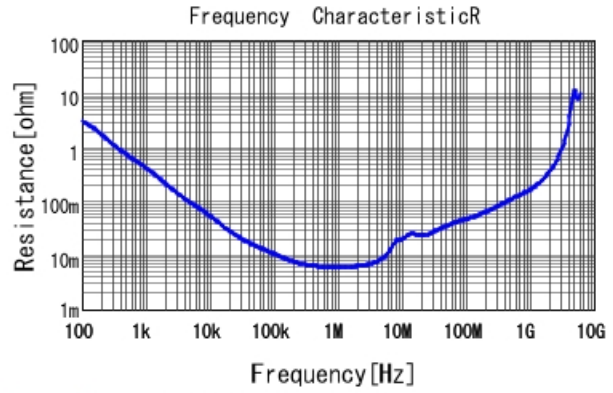
GRM319R61A225KA01 R DCOV, 25degC
