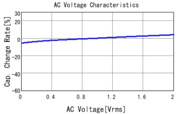
GRM319R61A225KA01 C-AC Voltage capchange, DCOV, 25
