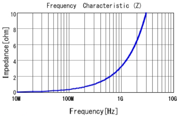
LQP03TG0N5C02 |Z|
