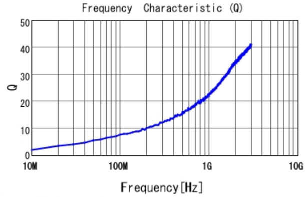
LQP03TG0N5C02 Q
