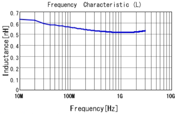
LQP03TG0N5C02 L
