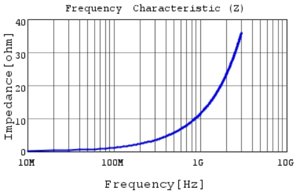
LQG15WZ1N8C02 |Z|
