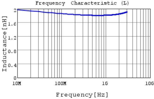
LQG15WZ1N8C02 L
