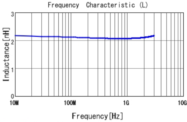
LQP03HQ2N0B02 L
