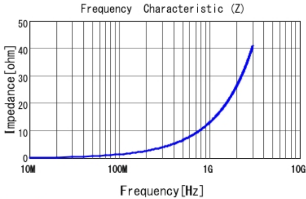
LQP03HQ2N0B02 |Z|
