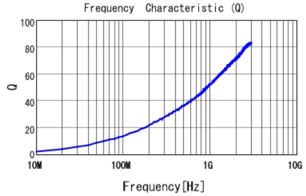
LQP03HQ2N0B02 Q
