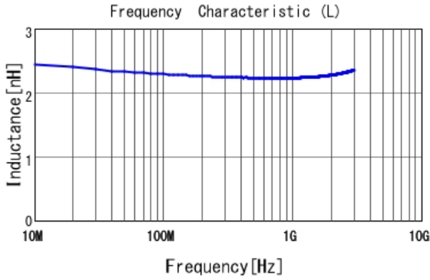
LQP03HQ2N2C02 L
