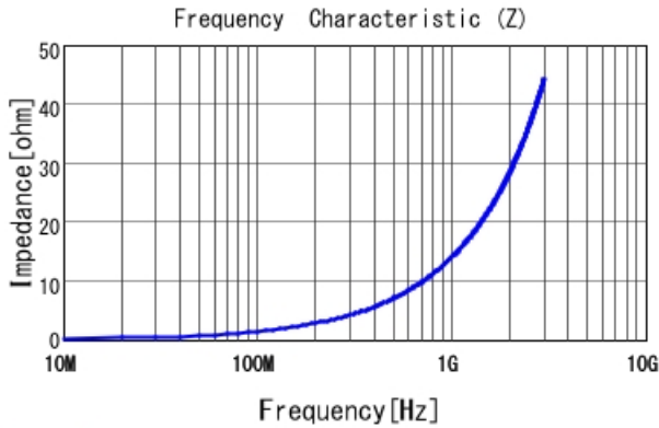
LQP03HQ2N2C02 |Z|
