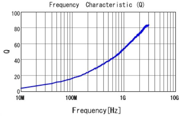
LQP03HQ2N2C02 Q
