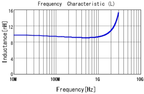
LQP03TG9N1H02 L
