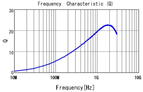
LQP03TG9N1H02 Q
