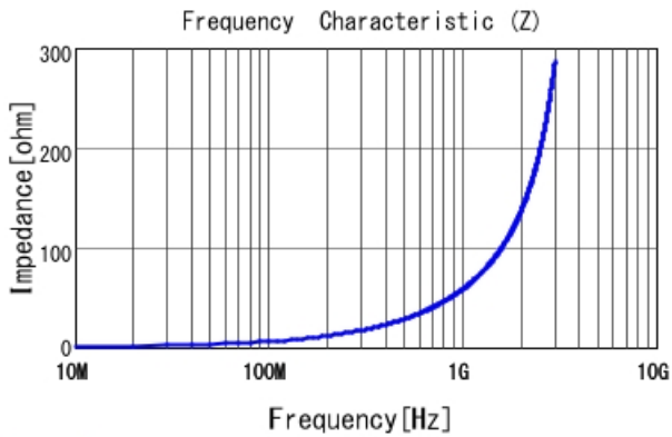
LQP03TG9N1H02 |Z|
