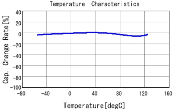
GRM188R71H102KA01 C-Temp. capchange, DC0.0V, AC1.C
