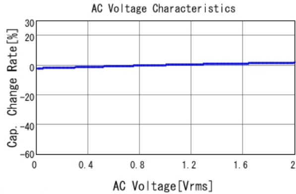
GRM188R71H102KA01 C-AC Voltage capchange, DCOV, 25
