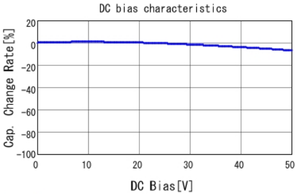
GRM188R71H102KA01 C-DC bias capchange, 25.0degC, A
