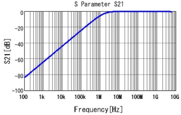
GRM188R71H102KA01 S21 DC0V, 25degC
