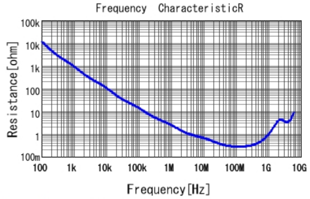
GRM188R71H102KA01 R DCOV, 25degC
