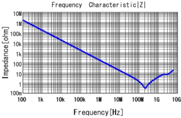
GRM188R71H102KA01 |Z| DCOV, 25degC
