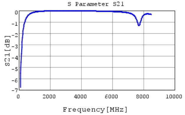
GCQ1555C1H8R2WB01 S21 DCOV, 25degC
