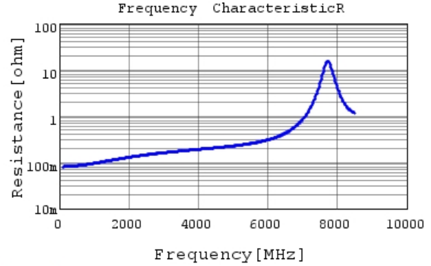
GCQ1555C1H8R2WB01 R DC0V, 25degC
