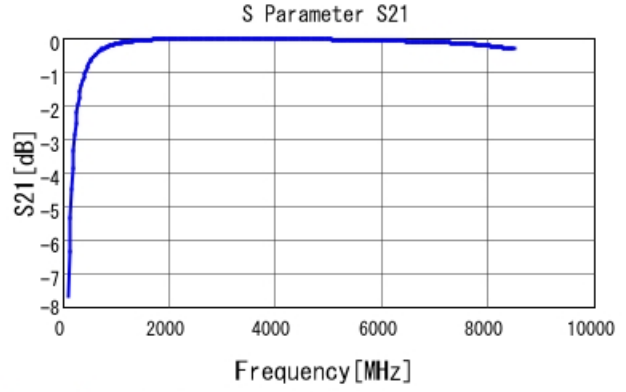
GJM1555C1H7R2BB01 S21 DC0V, 25degC
