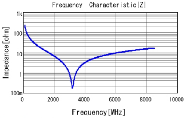
GJM1555C1H7R2BB01 |Z| DCOV, 25degC
