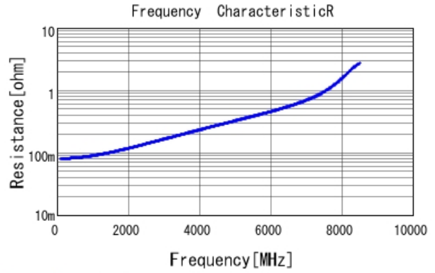
GJM1555C1H7R2BB01 R DCOV, 25degC
