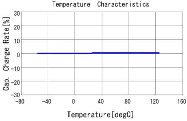
GJM1555C1H7R2BB01 C-Temp. capchange, DC0V, AC1Vrms
