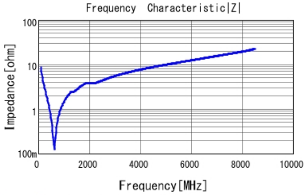
GRM1555C1E181JA01 |Z| DCOV, 25degC
