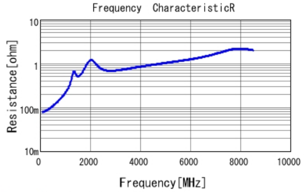
GRM1555C1E181JA01 R DCOV, 25degC
