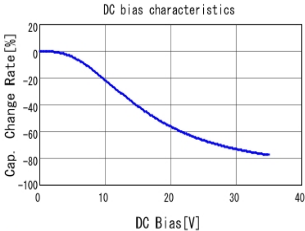
■ GRM219R7YA105MA12 C-DC bias capchange, 25.0degC, AC1.
