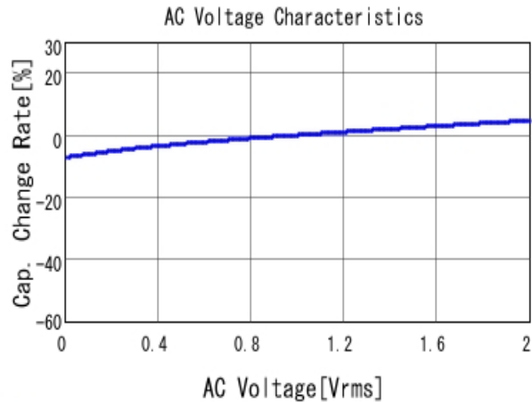
■ GRM219R7YA105MA12 C-AC Voltage capchange, DCOV, 25.0d
