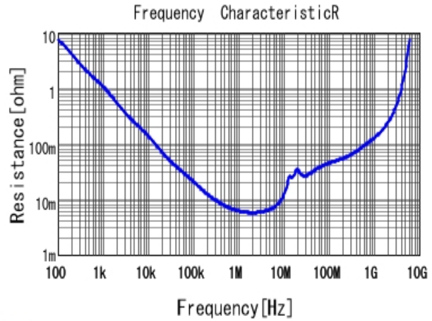
■ GRM219R7YA105MA12 R DCOV, 25degC
