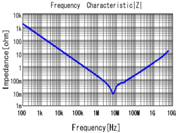
■ GRM219R7YA105MA12 |Z| DCOV, 25degC
