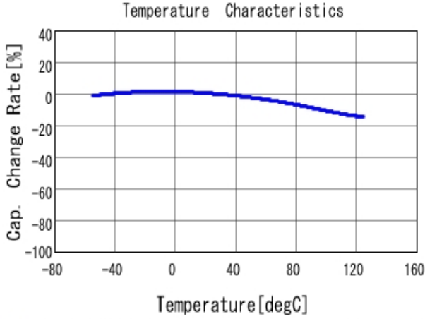
■ GRM219R7YA105MA12 C-Temp. capchange, DC0.0V, AC1.0V r m
