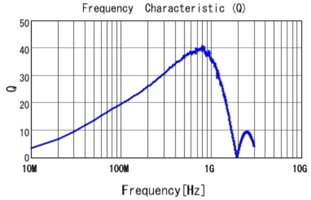
LQW15ANR10J00 Q
