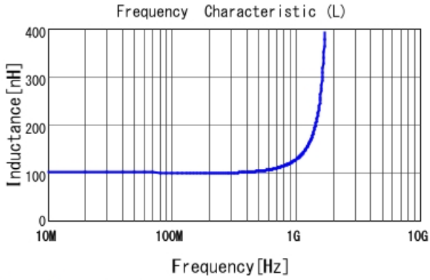
LQW15ANR10J00 L
