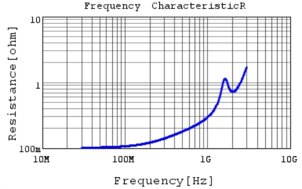
RCE5C1H820J0DBH03A R DCOV, 25degC
