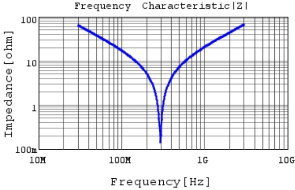
RCE5C1H820J0DBH03A |Z| DCOV, 25degC
