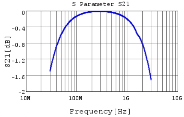
RCE5C1H820J0DBH03A S21 DCOV, 25degC
