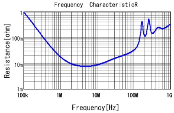
GRM21B5C2E682JWAA R DCOV, 25degC
