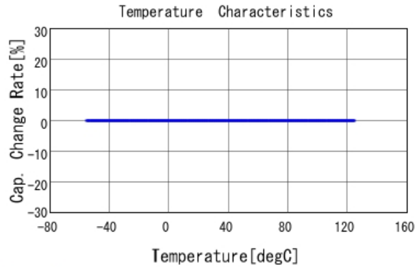
GRM21B5C2E682JWAA C-Temp. capchange, DCOV, AC1Vrms
