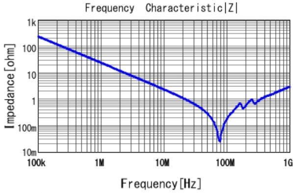
GRM21B5C2E682JWAA |Z| DCOV, 25degC
