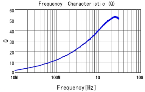
LQP03HQ6N8H02 Q
