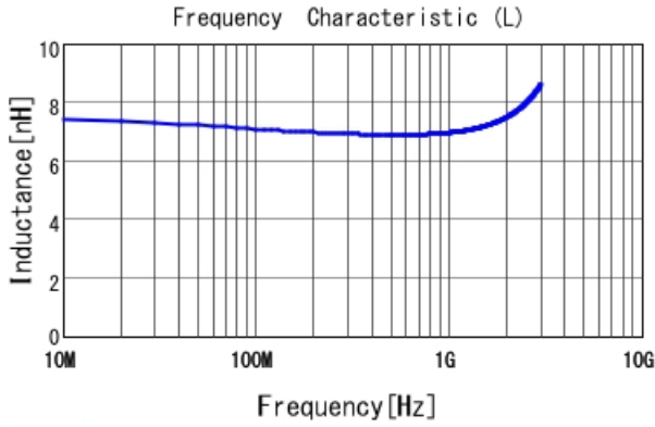
LQP03HQ6N8H02 L
