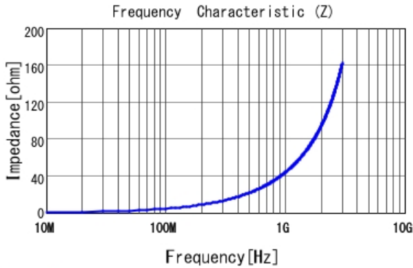
LQP03HQ6N8H02 |Z|
