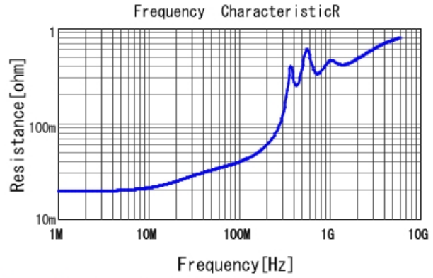
GRM1885C2A152JA01 R DCOV, 25degC
