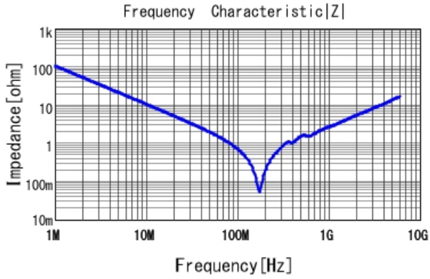
GRM1885C2A152JA01 |Z| DCOV, 25degC
