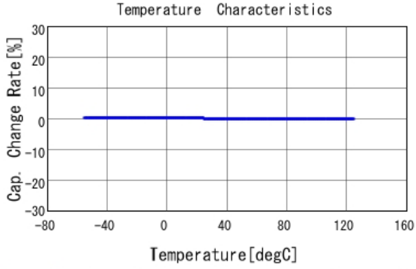
GRM1885C2A152JA01 C-Temp. capchange, DCOV, AC1Vrms
