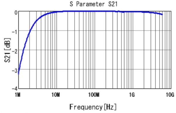
GRM1885C2A152JA01 S21 DCOV, 25degC
