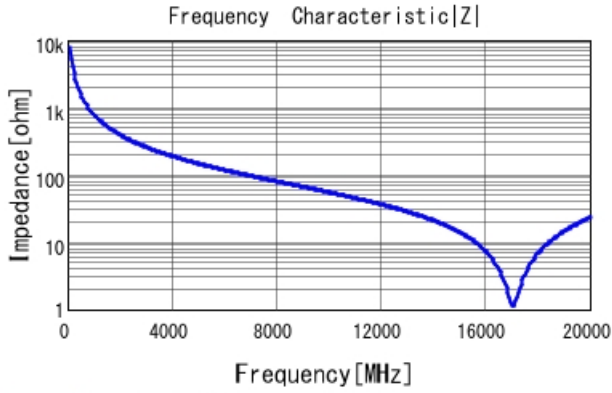
GRM1555C1HR20BA01 |Z| DCOV, 25degC
