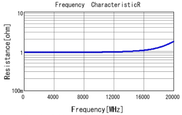
GRM1555C1HR20BA01 R DCOV, 25degC
