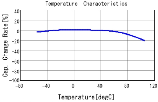
GRM21BC80J226ME51 C-Temp. capchange, DC0.0V, AC0.5
