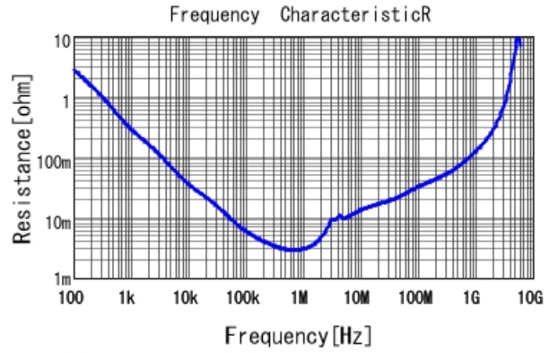
GRM21BC80J226ME51 R DCOV, 25degC
