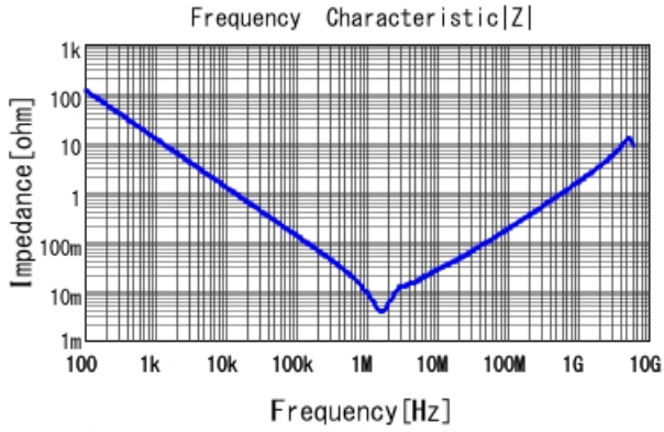
GRM21BC80J226ME51 |Z| DCOV, 25degC
