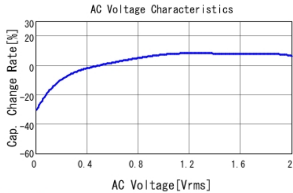
GRM21BC80J226ME51 C-AC Voltage capchange, DCOV, 25
