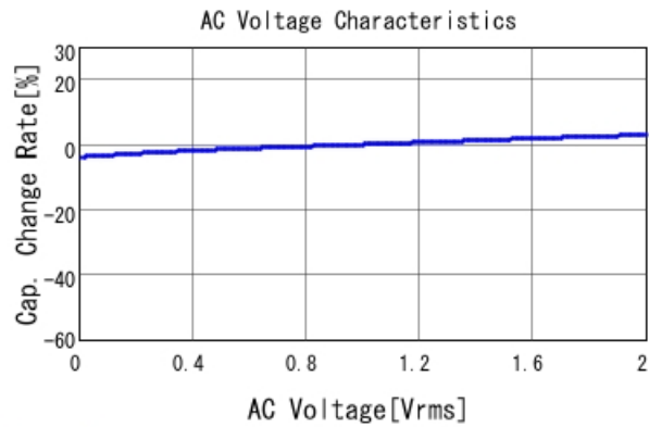
GCM155R71H153KA55 C-AC Voltage capchange, DCOV, 25
