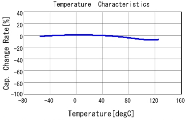
GCM155R71H153KA55 C-Temp. capchange, DC0.0V, AC1.C
