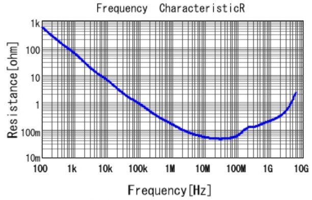
GCM155R71H153KA55 R DCOV, 25degC
