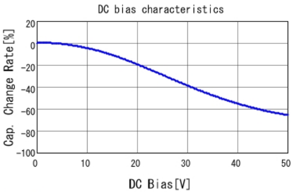
GCM155R71H153KA55 C-DC bias capchange, 25.0degC, A
