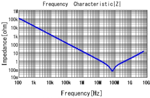
GCM155R71H153KA55 |Z| DCOV, 25degC
