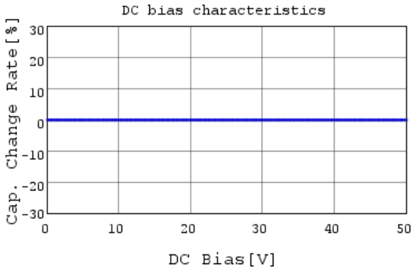
GCQ1555C1H5R8BB01 C-DC bias capchange, 25.0c
