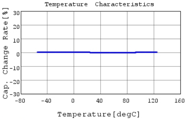
GRM3195C2A333JA01 C-Temp. capchange, DCOV, 1
