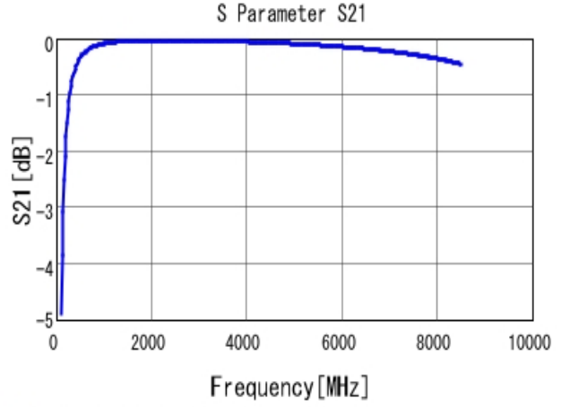
■ GRM0335C1H110JA01 S21 DCOV, 25degC
