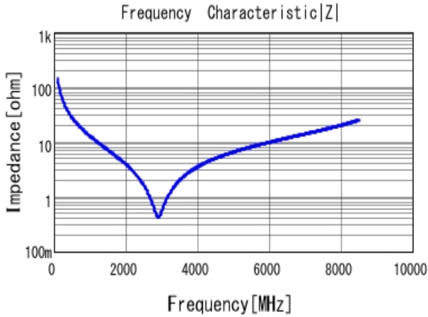
■ GRM0335C1H110JA01 |Z| DC0V, 25degC
