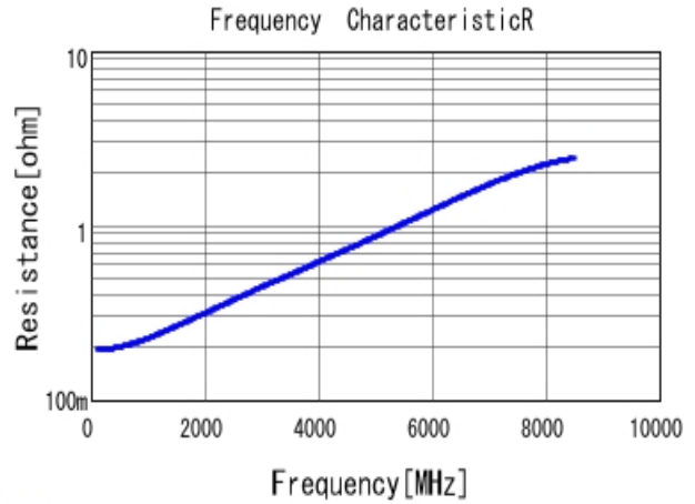
■ GRM0335C1H110JA01 R DC0V, 25degC
