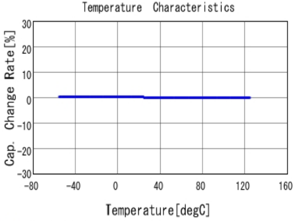
■ GRM0335C1H110JA01 C-Temp. capchange, DCOV, AC1Vrms
