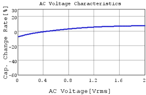
GRM033R61A333ME84 C-AC Voltage capchange, Dc
