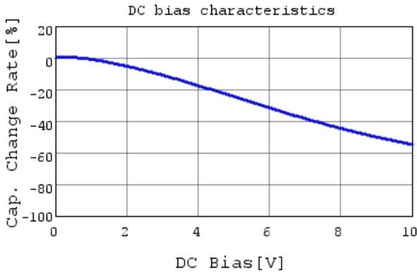
GRM033R61A333ME84 C-DC bias capchange, 25.0c
