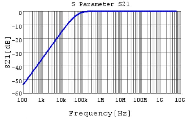
GRM033R61A333ME84 S21 DC0V, 25degC
