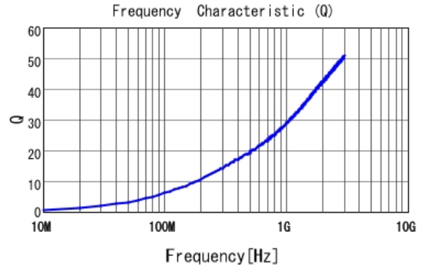
LQP15MN1N6B02 Q
