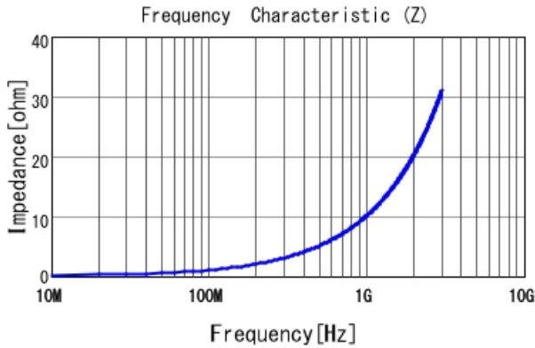
LQP15MN1N6B02 |Z|
