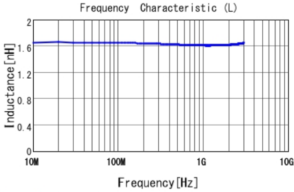
LQP15MN1N6B02 L
