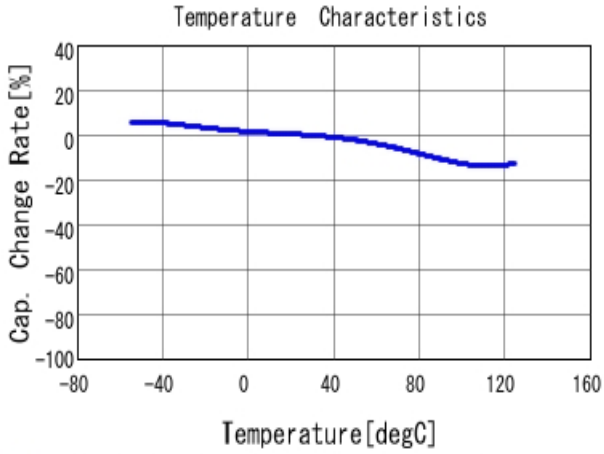
■ GRJ32DR72E224KWJ1 C-Temp. capchange, DCOV, AC1Vrms
