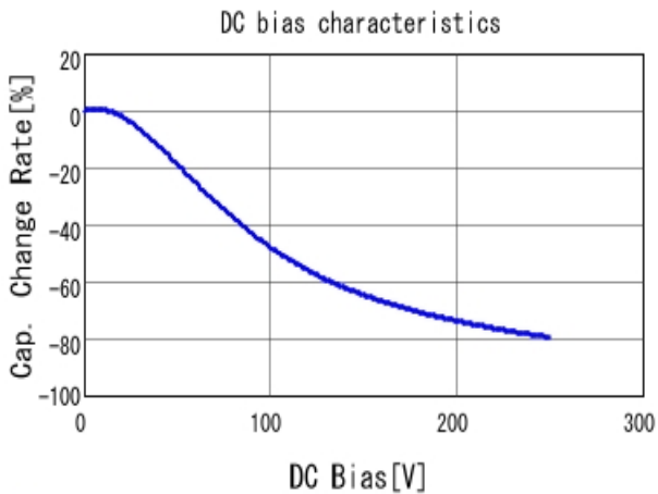
■ GRJ32DR72E224KWJ1 C-DC bias capchange, 25.0degC, AC1V
