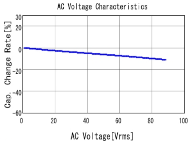
■ GRJ32DR72E224KWJ1 C-AC Voltage capchange, DCOV, 25.0d
