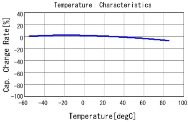
GRM155R61H104ME14 C-Temp. capchange, DC0.0V, AC1.C
