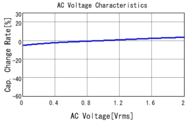
GRM155R61H104ME14 C-AC Voltage capchange, DCOV, 25
