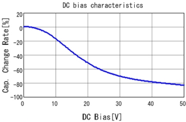
GRM155R61H104ME14 C-DC bias capchange, 25.0degC, A
