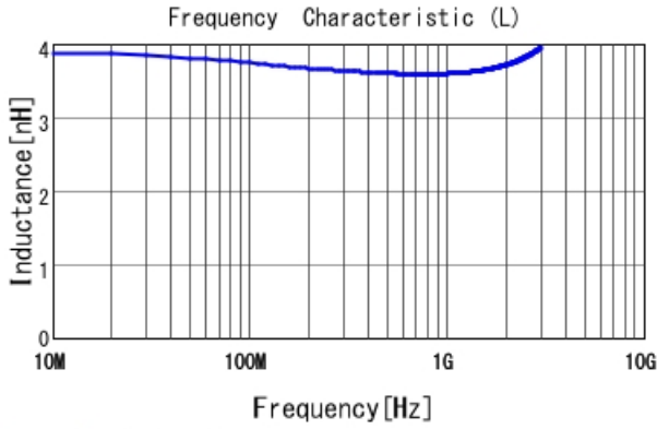
LQP15MN3N6B02 L
