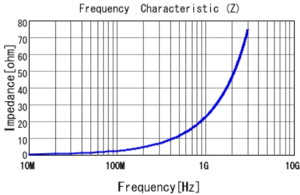
LQP15MN3N6B02 |Z|
