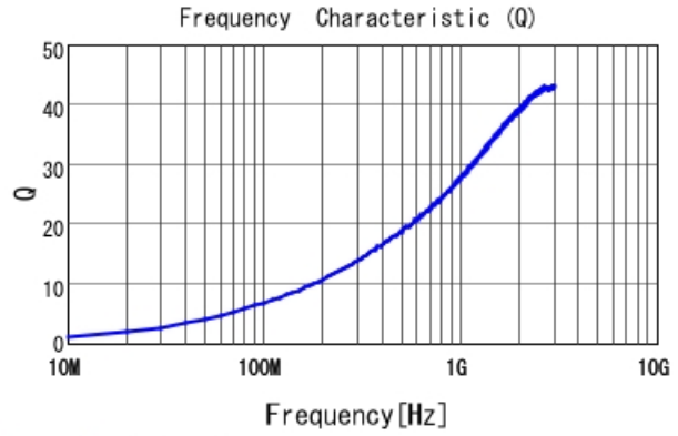
LQP15MN3N6B02 Q
