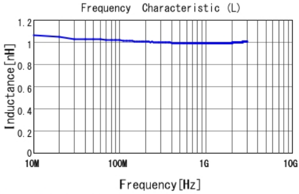
LQG15HN1N0B02 L
