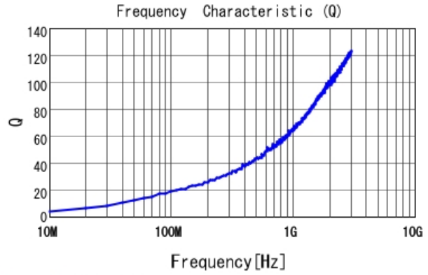
LQG15HN1N0B02 Q
