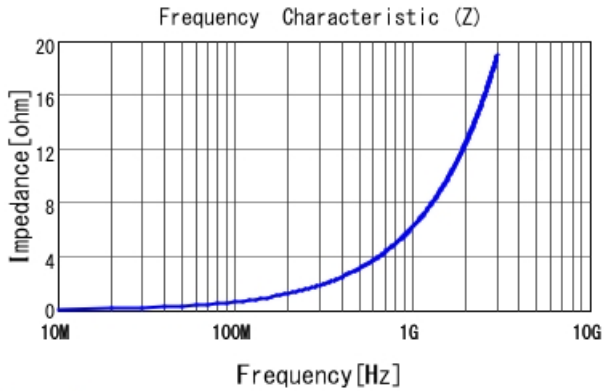
LQG15HN1N0B02 |Z|
