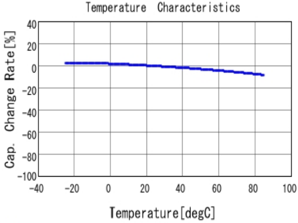
■ GRM21BB10J225KA01 C-Temp. capchange, DC0.0V, AC1.0V r m
