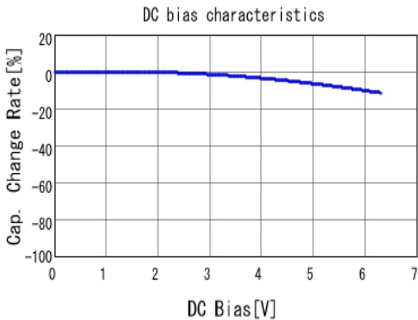
■ GRM21BB10J225KA01 C-DC bias capchange, 20.0degC, AC1.
