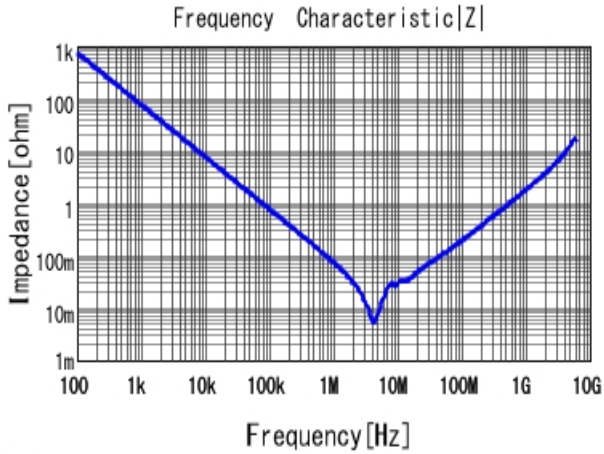
■ GRM21BB10J225KA01 |Z| DCOV, 20degC
