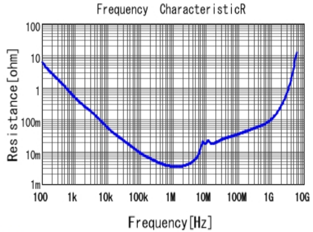
■ GRM21BB10J225KA01 R DCOV, 20degC
