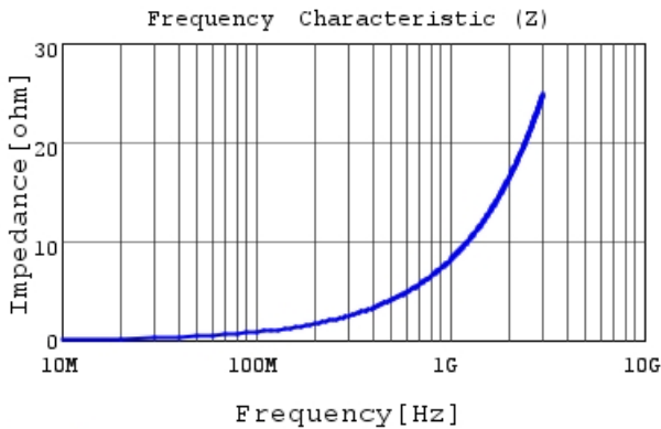
LQP15MN1N3B02 |Z|
