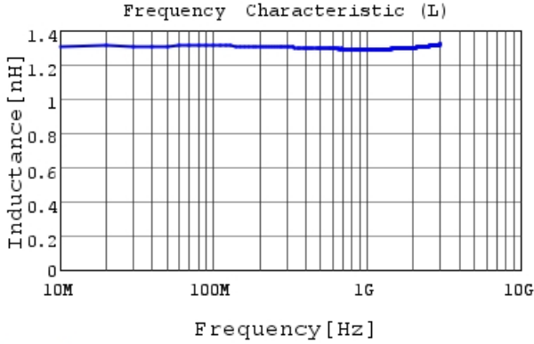
LQP15MN1N3B02 L
