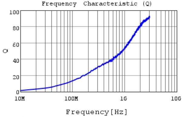
LQP15MN1N3B02 Q
