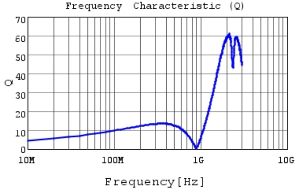
LQG15HSR10J02 Q
