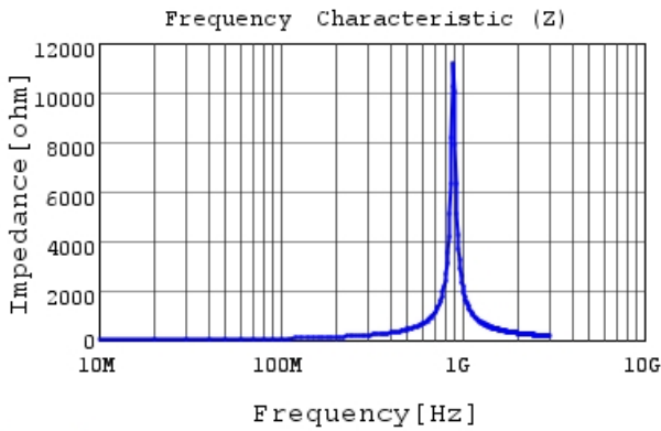
LQG15HSR10J02 |Z|
