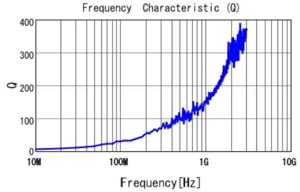
LQP03TQ0N6W02 Q
