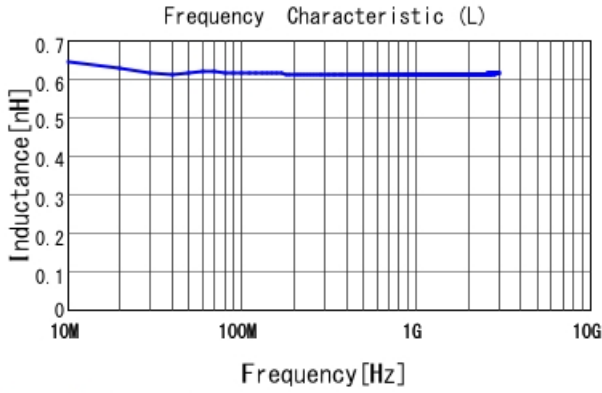
LQP03TQ0N6W02 L
