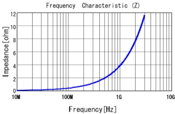
LQP03TQ0N6W02 |Z|
