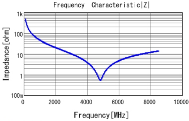
GCM1555C1H3R3CA16 |Z| DCOV, 25degC
