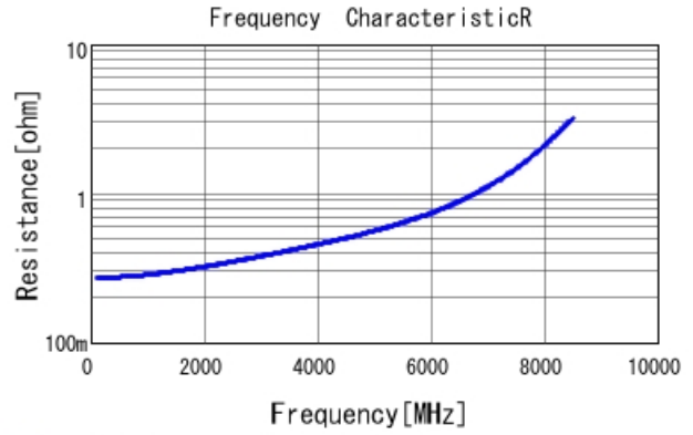
GCM1555C1H3R3CA16 R DCOV, 25degC
