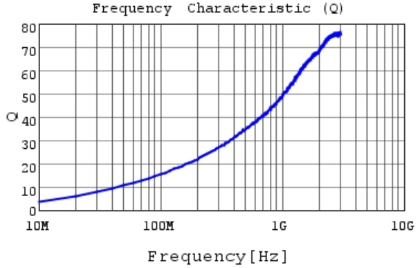
LQW04AN6N8D00 Q
