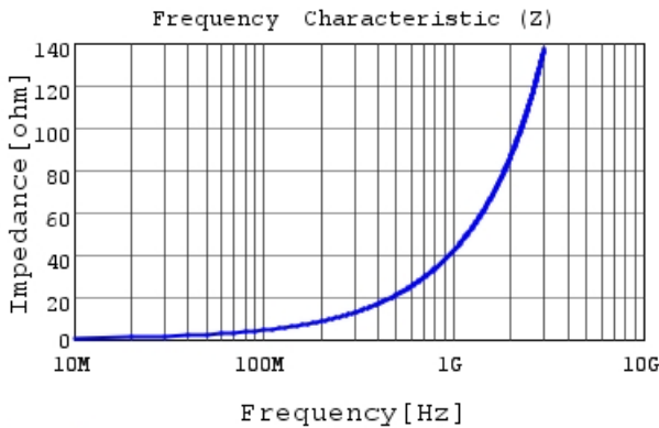
LQW04AN6N8D00 |Z|
