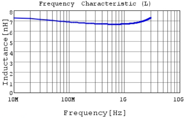
LQW04AN6N8D00 L
