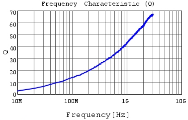
LQP03TQ2N6B02 Q
