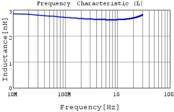
LQP03TQ2N6B02 L
