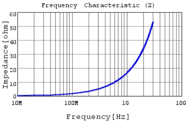
LQP03TQ2N6B02 |Z|
