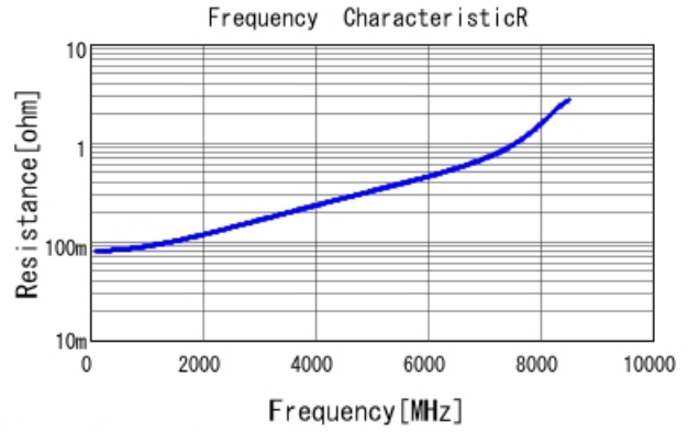
GJM1555C1H7R2CB01 R DCOV, 25degC
