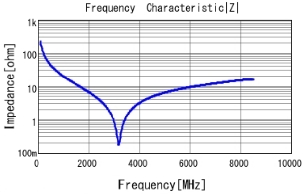
GJM1555C1H7R2CB01 |Z| DCOV, 25degC
