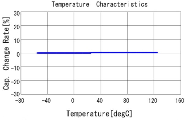
GJM1555C1H7R2CB01 C-Temp. capchange, DC0V, AC1Vrms
