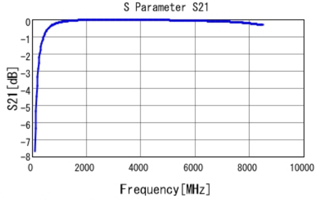
GJM1555C1H7R2CB01 S21 DC0V, 25degC
