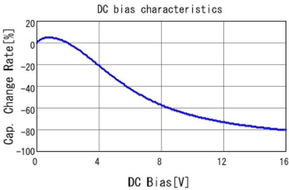
GCM155R71C154KE02 C-DC bias capchange, 25.0degC, A
