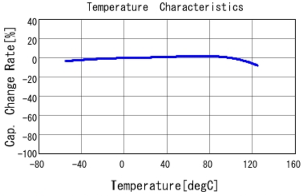
GCM155R71C154KE02 C-Temp. capchange, DC0.0V, AC1.C
