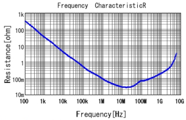
GCM155R71C154KE02 R DCOV, 25degC
