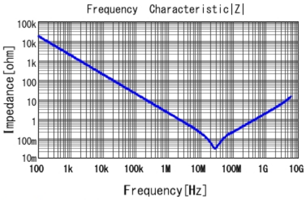
GCM155R71C154KE02 |Z| DCOV, 25degC
