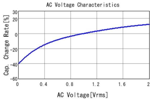
GCM155R71C154KE02 C-AC Voltage capchange, DCOV, 25
