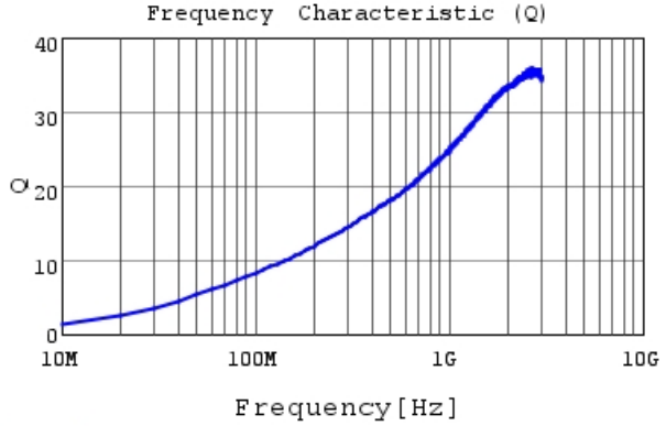
LQP02HQ12NJ02 Q
