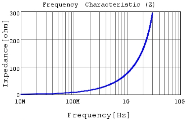
LQP02HQ12NJ02 |Z|
