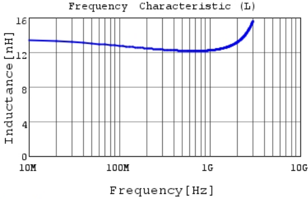
LQP02HQ12NJ02 L
