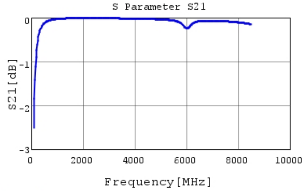
GJM0335C1E180GB01 S21 DCOV, 25degC
