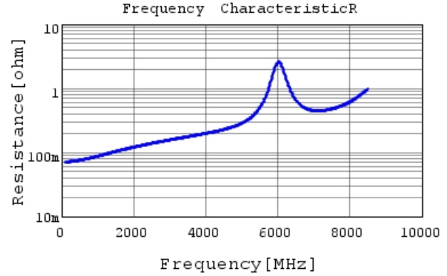
GJM0335C1E180GB01 R DC0V, 25degC
