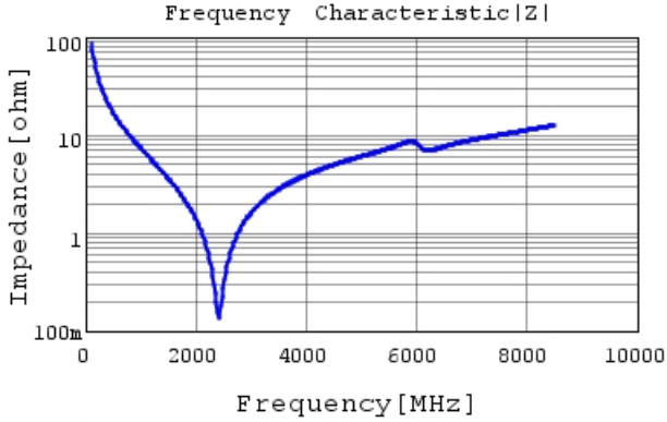
GJM0335C1E180GB01 |Z| DC0V, 25degC
