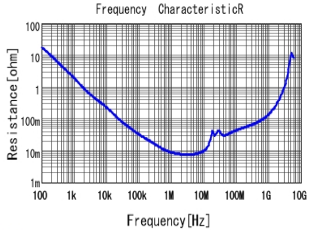
■ GRM21BR71H474KA88 R DCOV, 25degC
