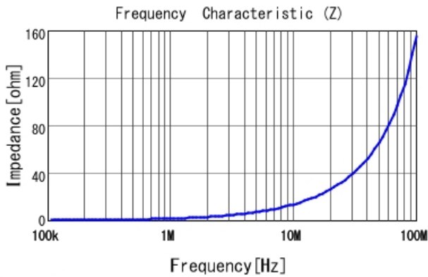
DFE201612P-R24M |Z|
