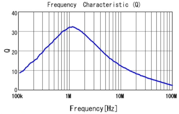
DFE201612P-R24M Q
