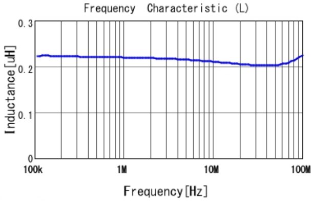
DFE201612P-R24M L
