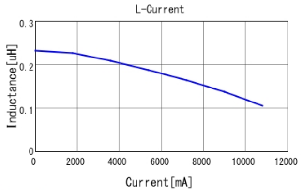
DFE201612P-R24M L-Current 20degC
